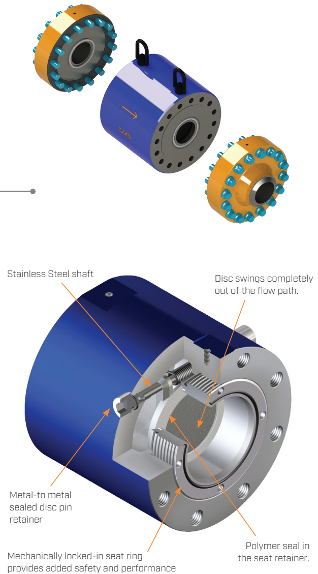
Typical “STC” Compact Check Valve
